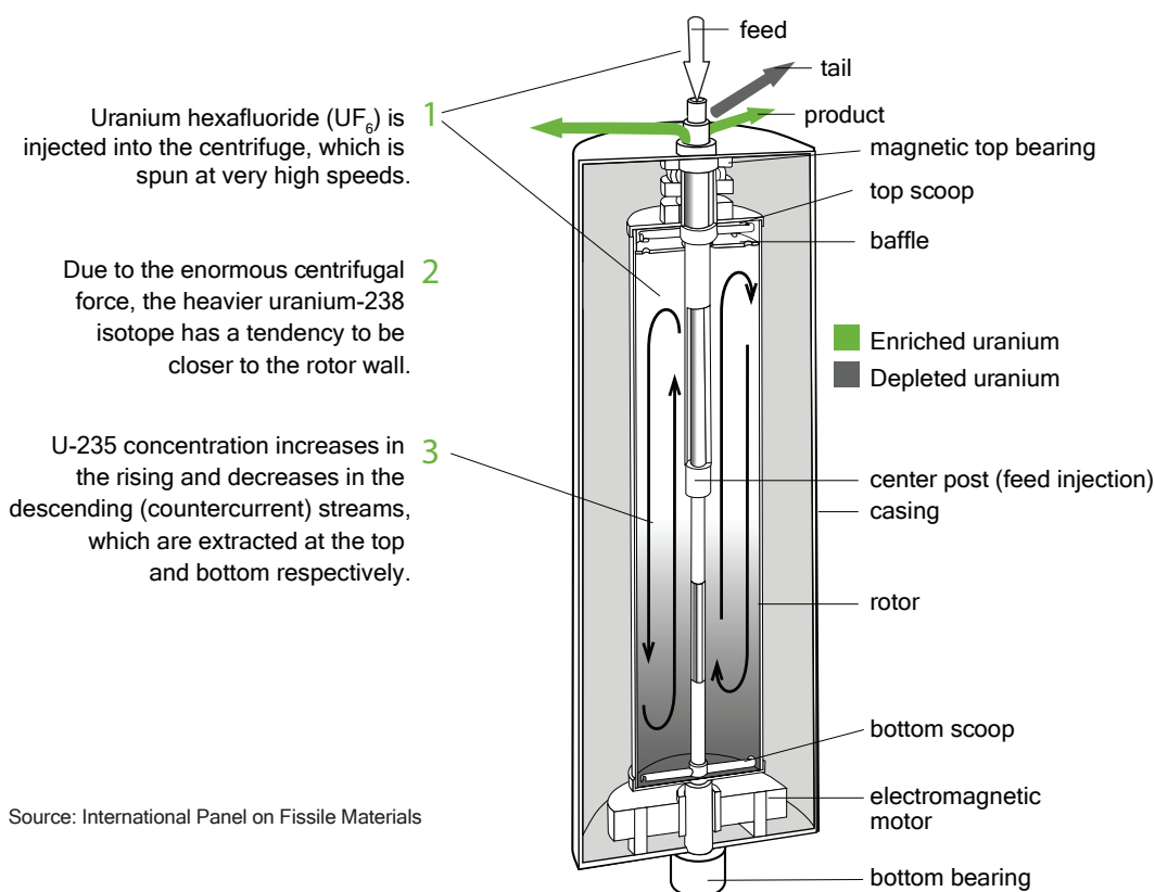
FIG 3: Gas centrifuge.
